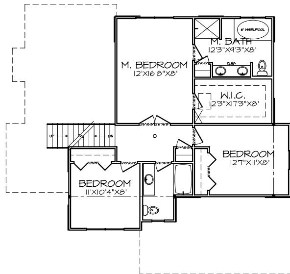
1 SECOND FLOOR PLAN A-5
