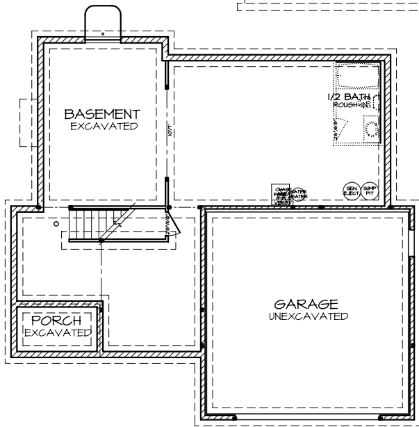
1 FOUNDATION PLAN A-3
